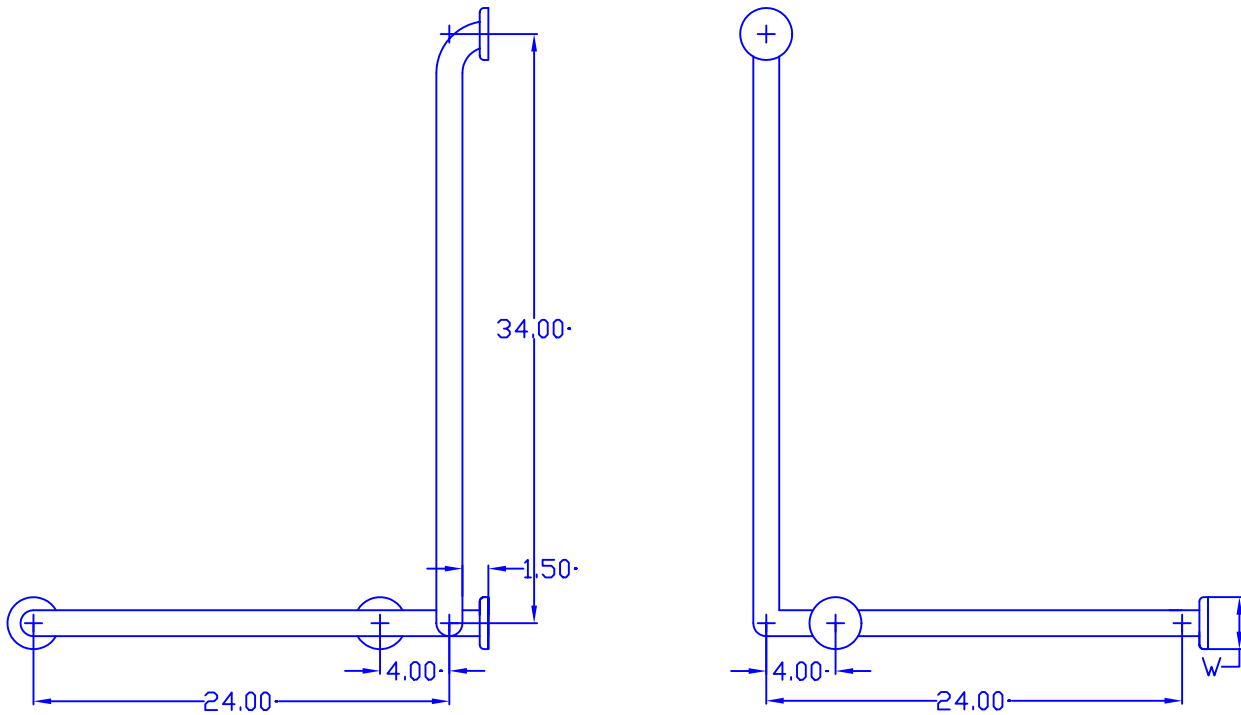
(2) PIECE CONSTRUCTION RIGHT HAND MODEL SHOWN
